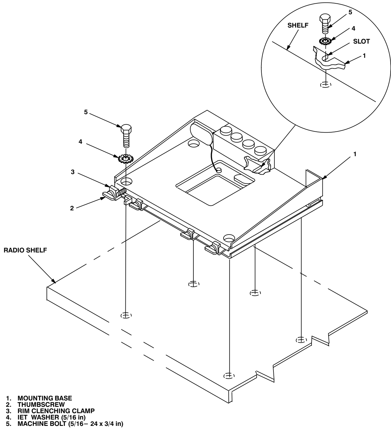
Figure 5-4. Mounting Base Installation
