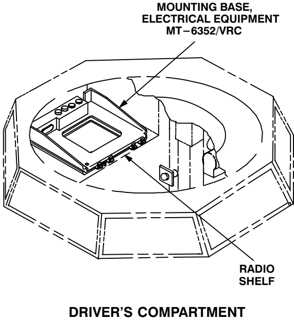
Figure 5-1 (1). MK and Radio Installation: MK Equipment Locations
